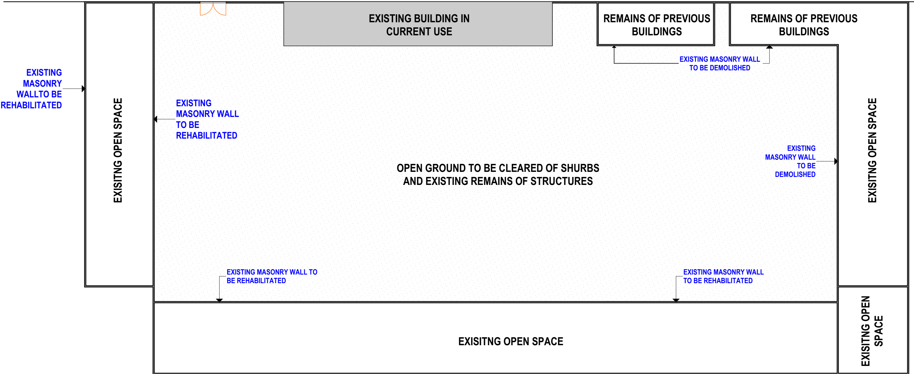
EXISTING SITE LAYOUT - KISMAYO WATER MINISTRY BUILDINGS
