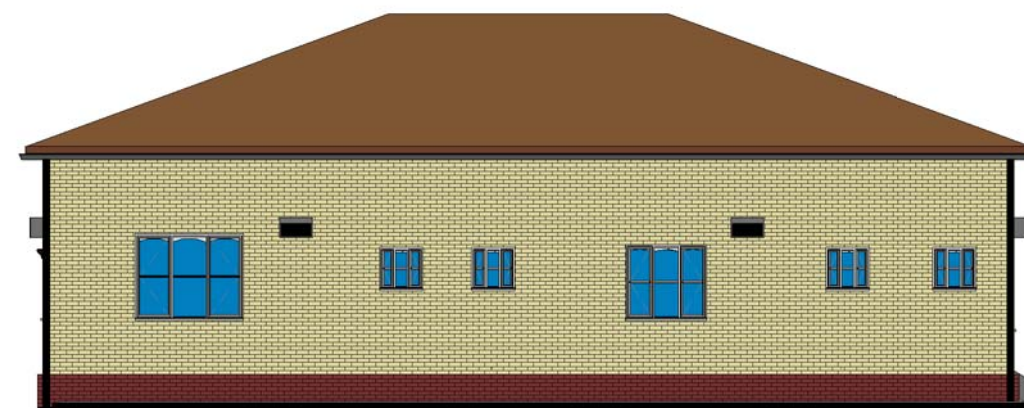
WEST ELEVATION
