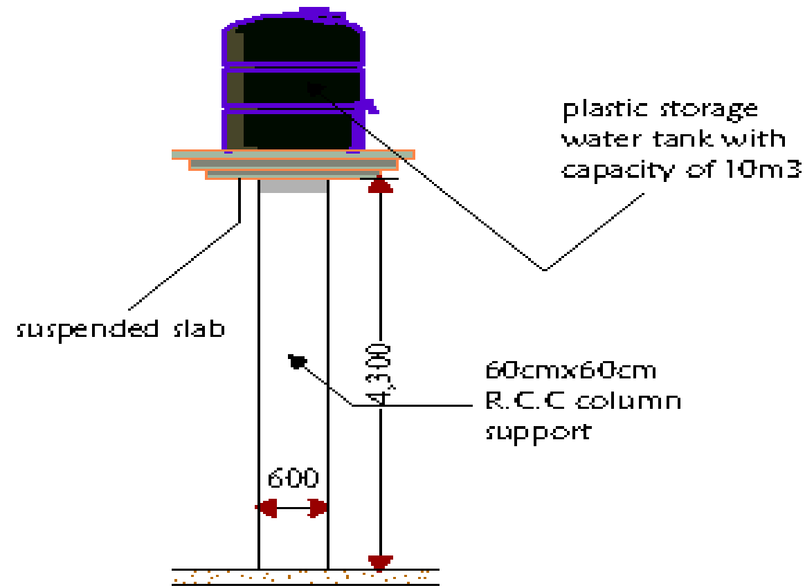
Elevated water tank -Elevation-
