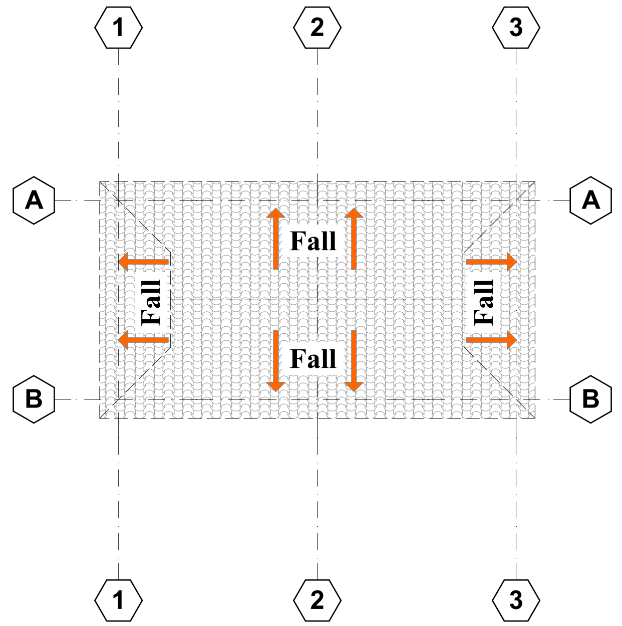
Roof Plan
