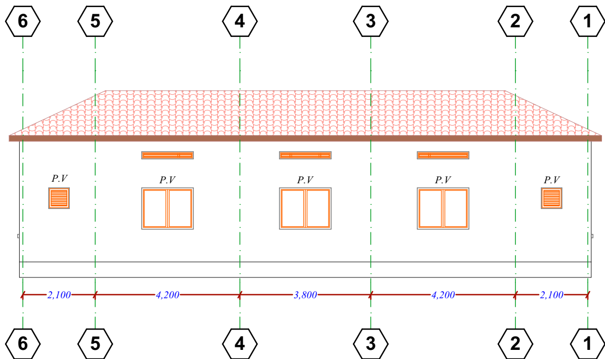
Elevation 03
